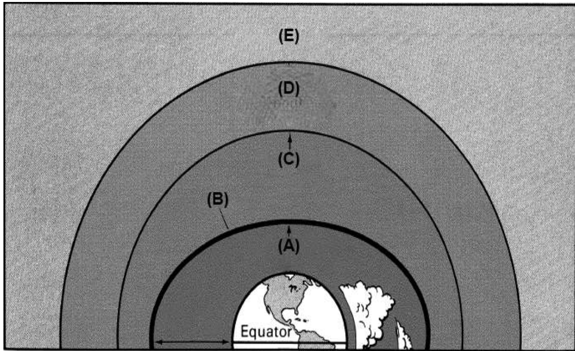
Figure 1 - Atmospheric Layers
