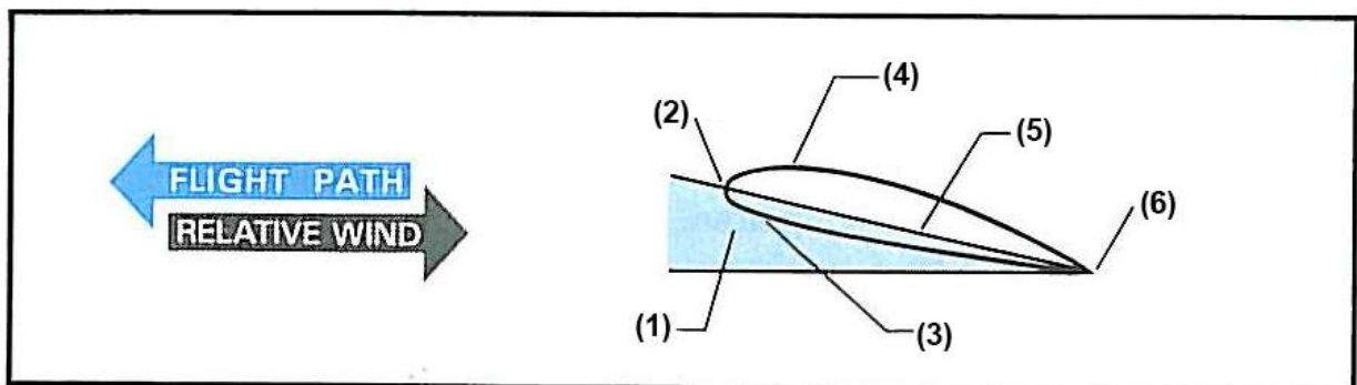
Figure 2 - Cross-section of a wing
